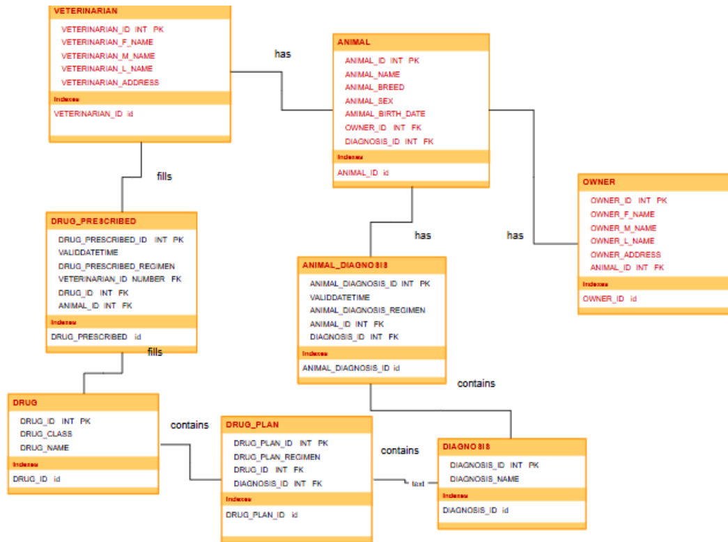
Fig: ER(Entity Relationship) diagram of PetBondhuBD app
